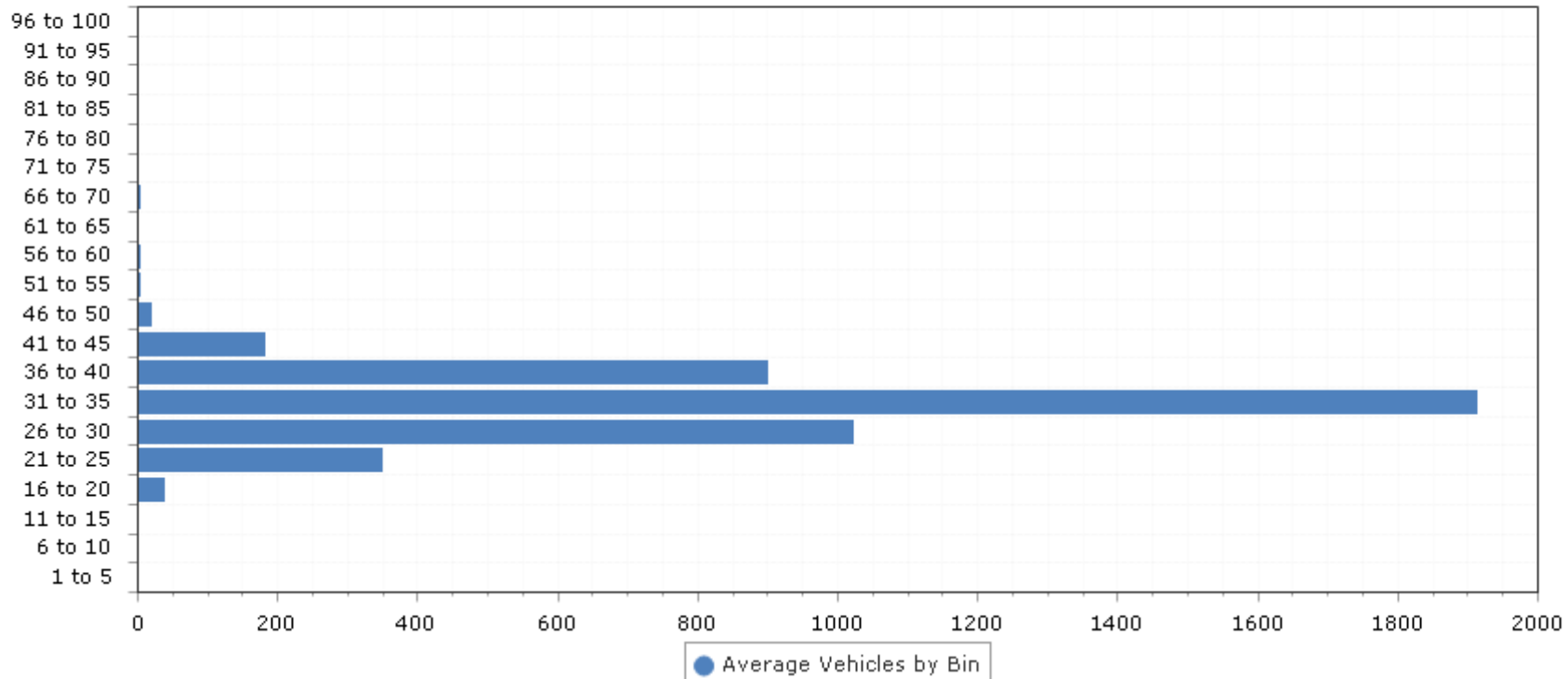
Average Vehicles per Day by Speed Bin
